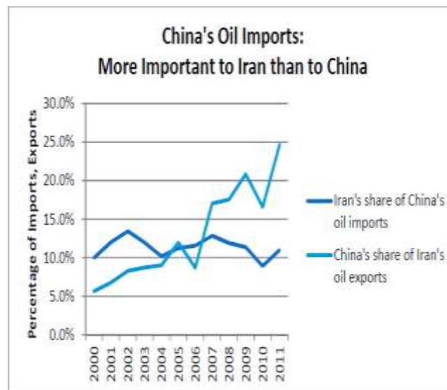
Figure 5: China's Oil Imports from 2000 to 2011: More Important to Iran than to China Source: IEA
