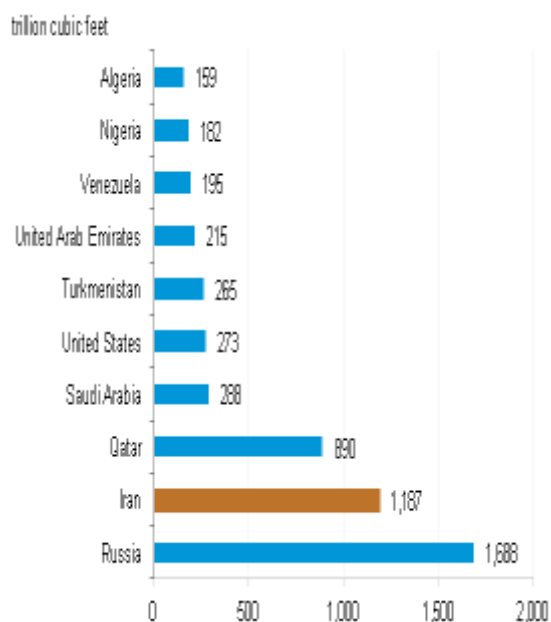
Figure 1: Largest proven reserve holders of natural gas, January 2013
